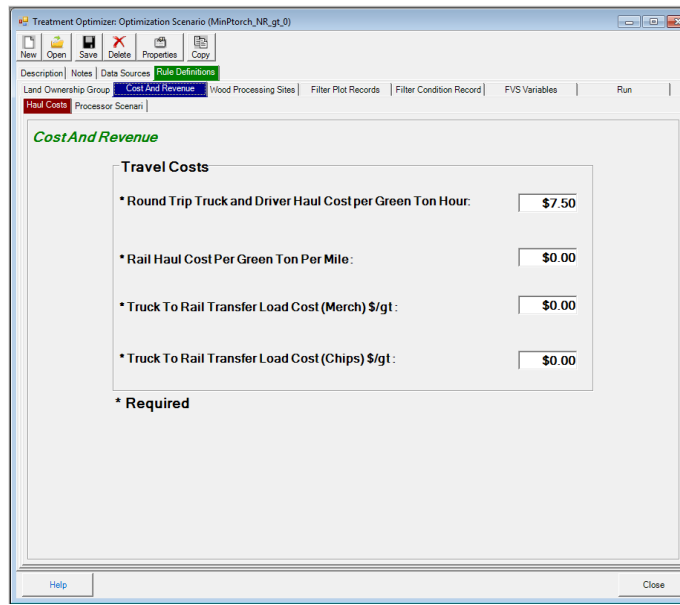
Figure 6.10: Haul Costs child tab on the Costs and Revenue tab
