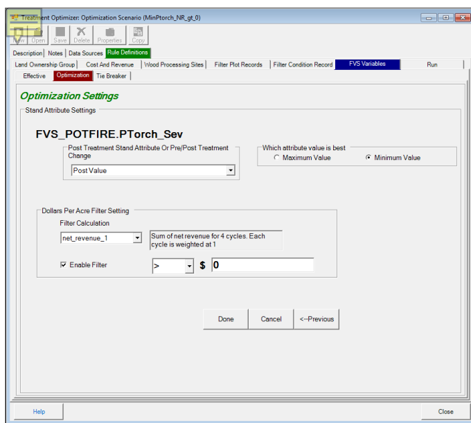
Figure 6.18: Follow-on stand attribute settings configuration window
