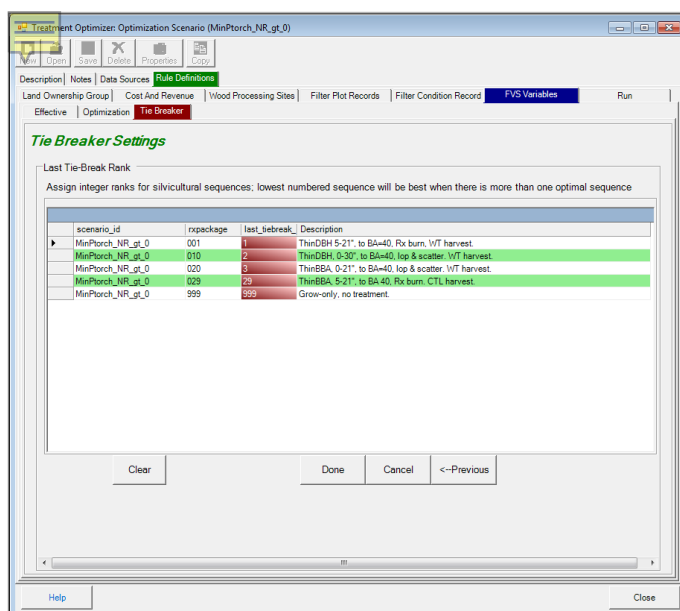
Figure 6.21: The Last Tie-Break Rank window
